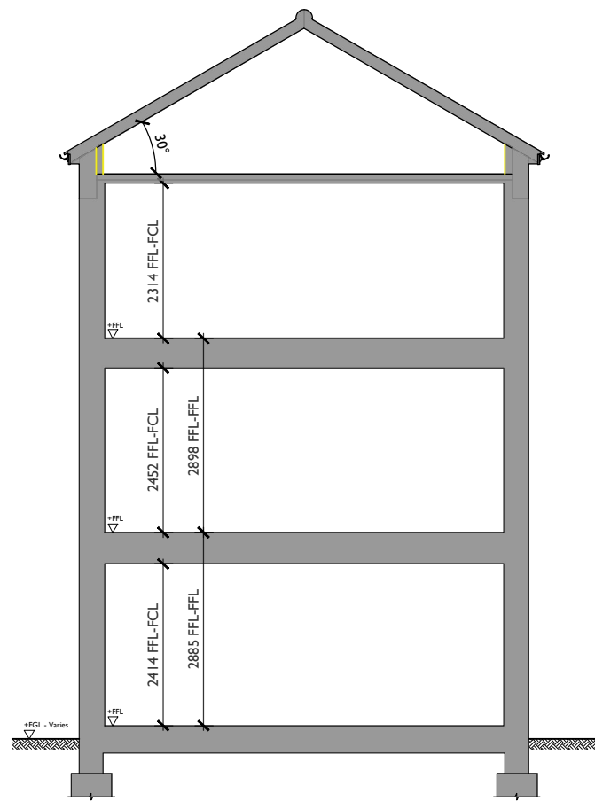
Plot 148-153 - Section S30-3-3.2 Truss Type F-30°
