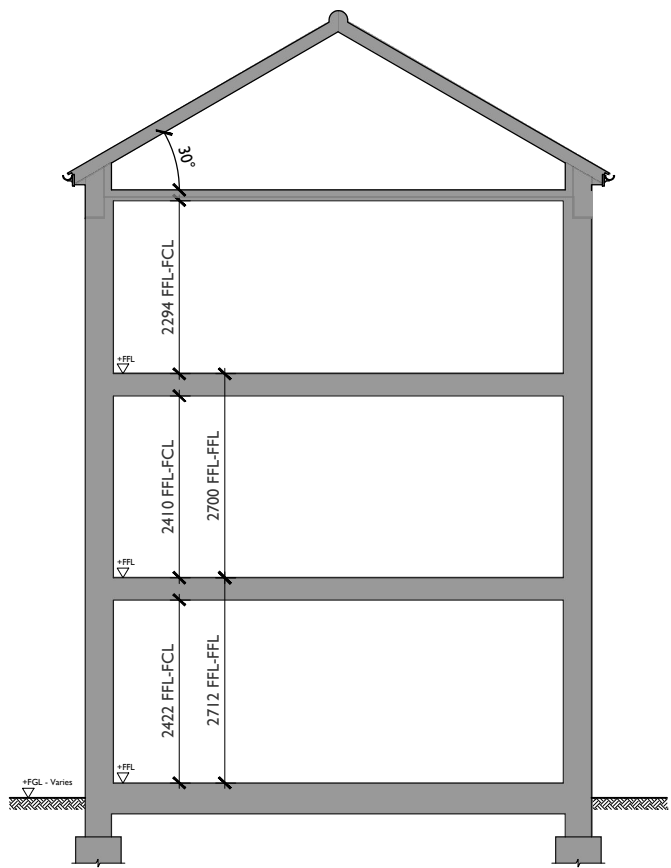
Plot 154-156 - Section S30-3-3.2 Truss Type F-30°
