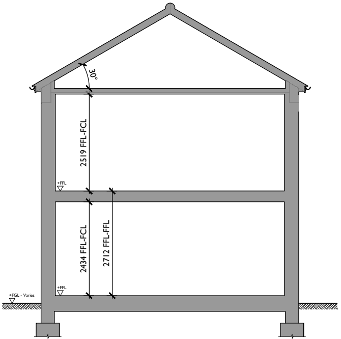
Plot 157-158 - Section Bespoke Truss Type F-30°
